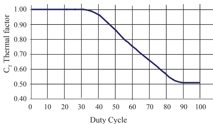
Chart 3 : Thermal Factor, C_T
