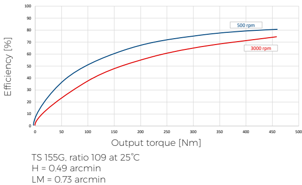
Fig. 3.13: Efficiency charts
