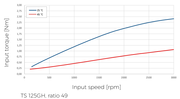
Fig. 3.16: No-load running torque charts
