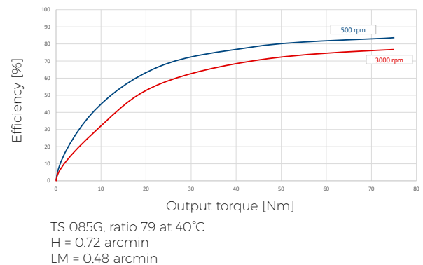
Fig. 3.13: Efficiency charts
