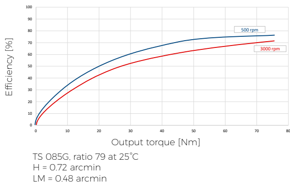
Fig. 3.13: Efficiency charts
