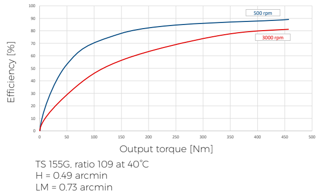
Fig. 3.13: Efficiency charts
